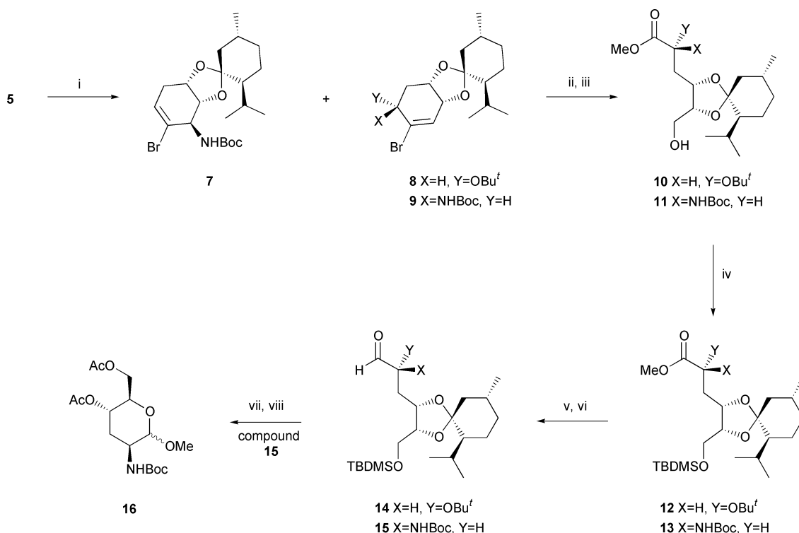
Scheme 2 Reagents and conditions: (i) AgOCN (7.0 mol equiv.), Bu t OH, 80 °C, 72 h; (ii) O 3 , CH 2 Cl 2 -MeOH, pyridine (4.0 mol equiv.), -90 °C, 0.2 h; (iii) KI (1.5 mol equiv.), NaBH 4 (6.0 mol equiv.), -90-0 °C, 1 h; (iv) TBDMSOTf (1.5 mol equiv.), 2,6-dimethylpyridine, CH 2 Cl 2 , 0-18 °C, 0.5 h (for 10 → 12 ) or TBDMSOTf (1.3 mol equiv.), Et 3 N (1.8 mol equiv.), DMAP (trace), CH 2 Cl 2 , 18 °C, 7 h (for 11 → 13 ); (v) DIBAL-H (2.0 mol equiv.), CH 2 Cl 2 , -78-18 °C, 8 h; (vi) Dess-Martin reagent (1.5 mol equiv.), pyridine, CH 2 Cl 2 , 0-18 °C, 4 h; (vii) 36% HCl (trace) in MeOH, 0-18 °C, 18 h; (viii) Ac 2 O (mol equiv.), pyridine, 0-18 °C, 3 h.
