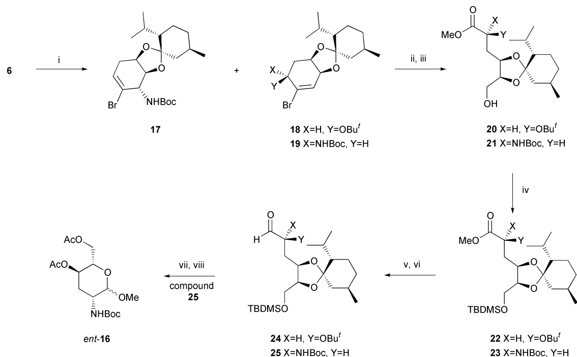
Scheme 3 Reagents and conditions: (i) AgOCN (7.0 mol equiv.), Bu t OH, 80 °C, 72 h; (ii) O 3 , CH 2 Cl 2 -MeOH, pyridine (4.0 mol equiv.), -90 °C, 0.2 h; (iii) KI (1.5 mol equiv.), NaBH 4 (6.0 mol equiv.), -90 to 0 °C, 1 h; (iv) TBDMSOTf (1.5 mol equiv.), 2,6-dimethylpyridine, CH 2 Cl 2 , 0-18 °C, 0.5 h (for 20 → 22 ) or TBDMSCl (1.3 mol equiv.), Et 3 N (1.8 mol equiv.), DMAP (trace), CH 2 Cl 2 , 18 °C, 7 h (for 21 → 23 ); (v) DIBAL-H (2.0 mol equiv.), CH 2 Cl 2 , -78-18 °C, 8 h; (vi) Dess-Martin reagent (1.5 mol equiv.), pyridine, CH 2 Cl 2 , 0-18 °C, 4 h; (vii) 36% HCl (trace) in MeOH, 0-18 °C, 18 h; (viii) Ac 2 O (mol equiv.), pyridine, 0-18 °C, 3 h.
