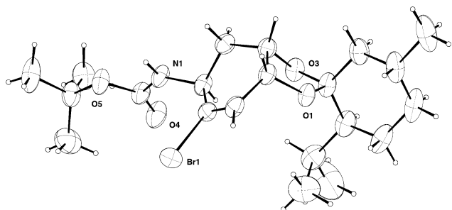
Fig. 1 ORTEP (with 50% probability ellipsoids) of compound 9 derived from X-ray crystallographic data.
