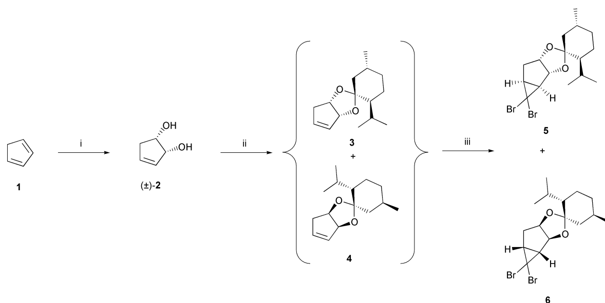
Scheme 1 Reagents and conditions: (i) \text{Pb}(\text{OCOMe})_4 (0.68 mol equiv.), \text{MeCO}_2\text{H} , \text{H}_2\text{O} , 0–18 °C, 1 h then \text{K}_2\text{CO}_3 , \text{MeOH} , 18 °C, 2 h; (ii) (–)-menthone (1.2 mol equiv.), p -TsOH (trace), pentane, 36 °C, 48 h then DBU (1.1 mol equiv. wrt p -TsOH); (iii) \text{CHBr}_3 , 50% aq. NaOH, \text{C}_6\text{H}_6 , TEAC, 0–18 °C, 48 h (TEAC = triethylbenzylammonium chloride).
